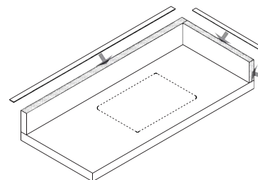
ASSEMBLY 2 Deck Mount, Manufacturer Assembled
